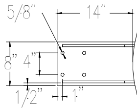
Bracket Detail
