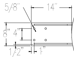
Bracket Detail
