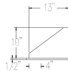
Bracket Detail
