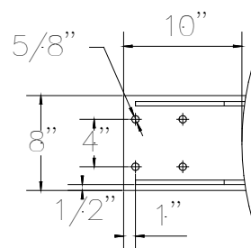
Bracket Detail
