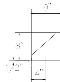
Bracket Detail
